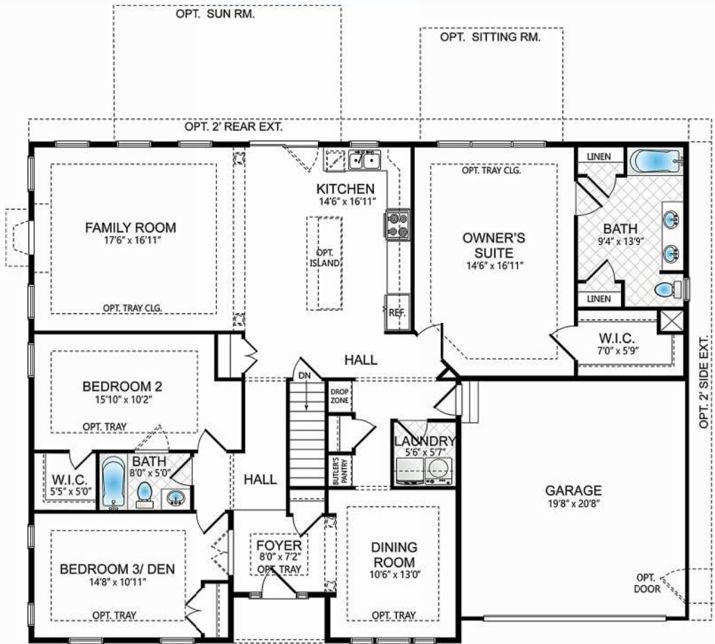
FIRST FLOOR PLAN ELEVATION - A
