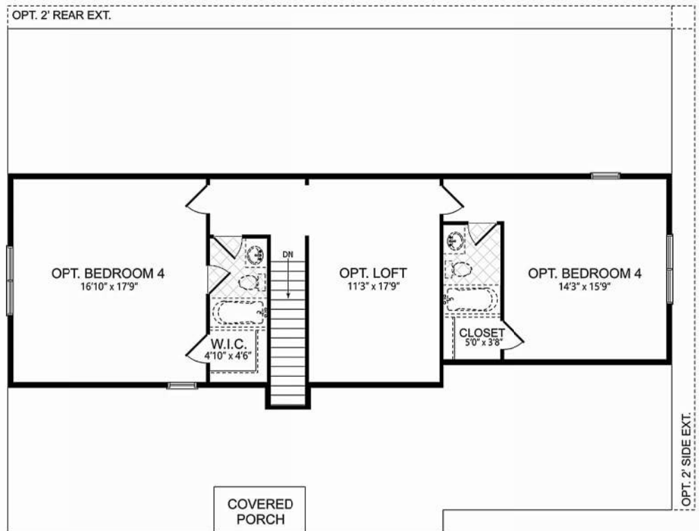
OPT. LOFT FLOOR PLAN W/BEDROOM 4 & 5 NOT AVAILABLE WITH ELEVATION D
